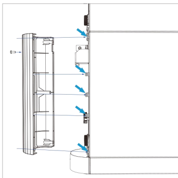
Installation of communication side decorative covers
