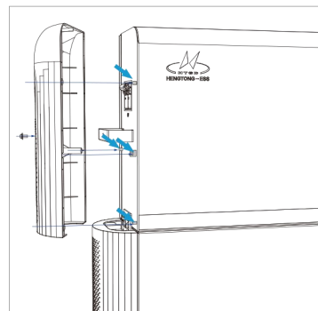
Installation of communication side decorative covers
